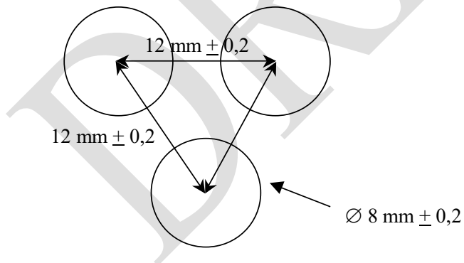
Top and bottom back plate flanges
