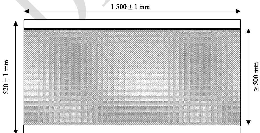
Figure 5 Design of the back plate
