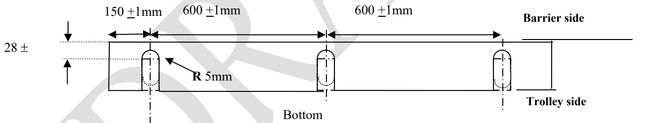
Figure 9 Ventilation frame
