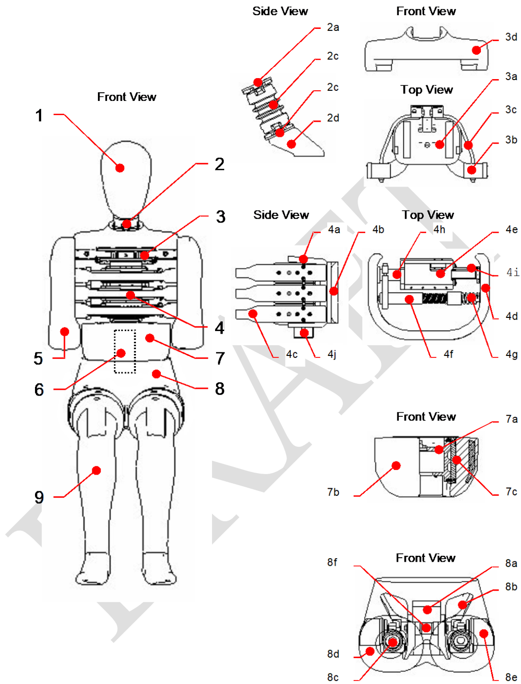
Figure 1 Construction of side impact dummy
