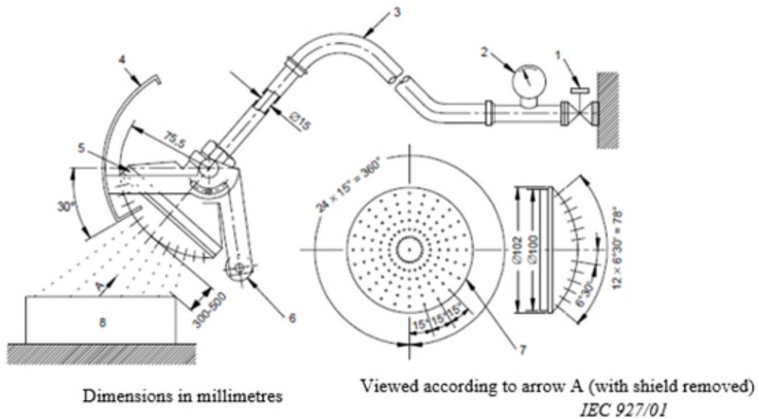
Figure 2 Splashing Test Nozzle
